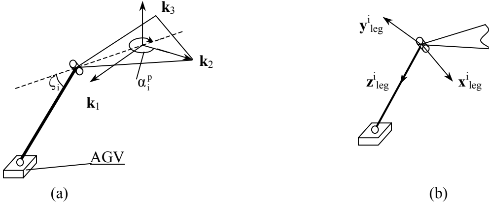
Figure 4. System with ball joint at the lower end of the leg and new leg frame.
