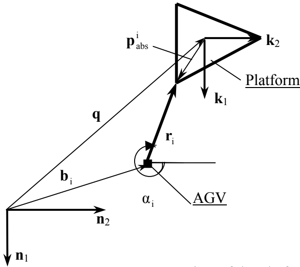
Figure 2. Top view of the platform (only one leg shown).
