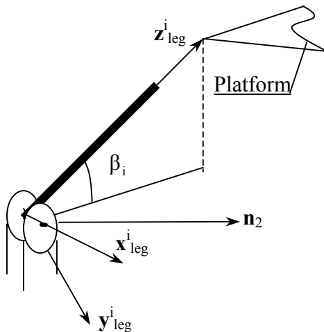
Figure 3. Revolute joint at lower end of the leg.
