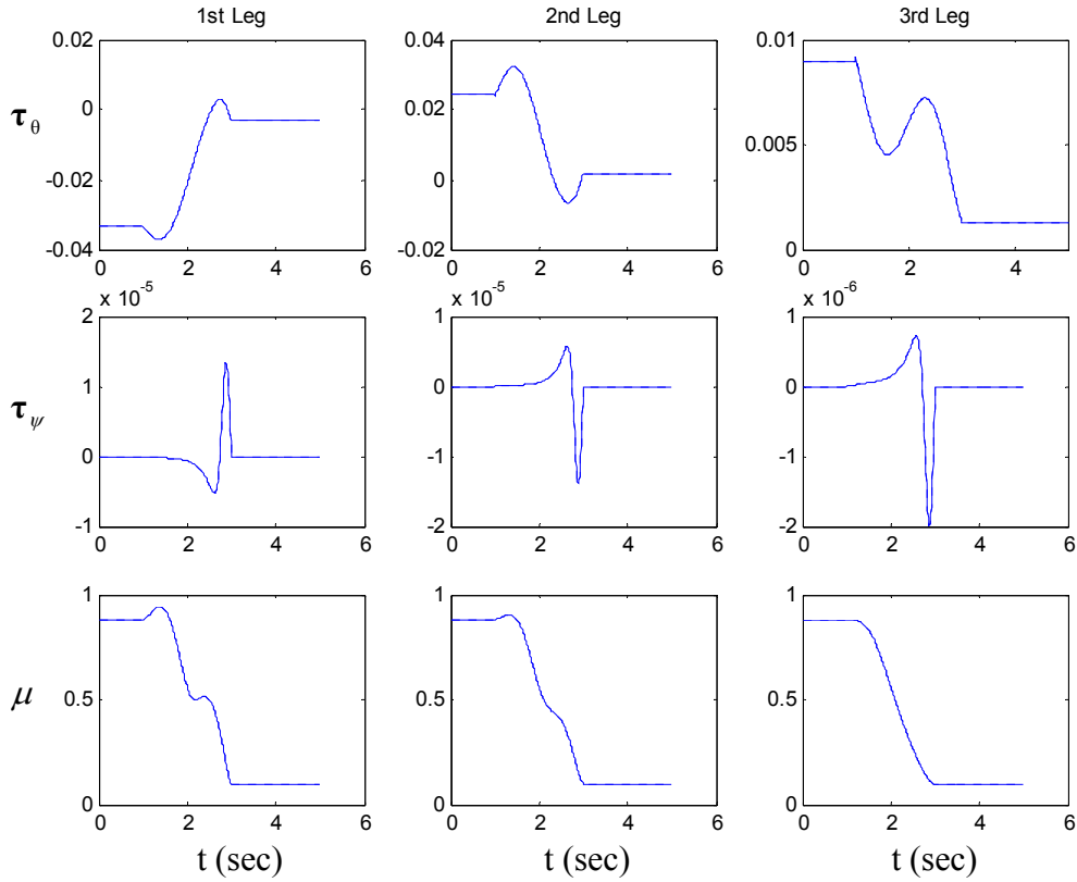
Figure 9. Required motor torques ( \tau_\theta and \tau_\psi ) and friction coefficient ( \mu ) for the three AGVs for the first maneuver.
