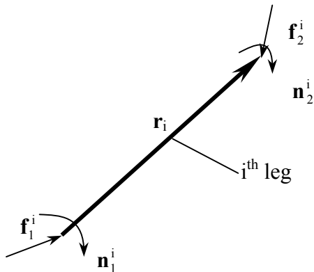
Figure 6. Free body diagram for the i^{\text{th}} leg.
