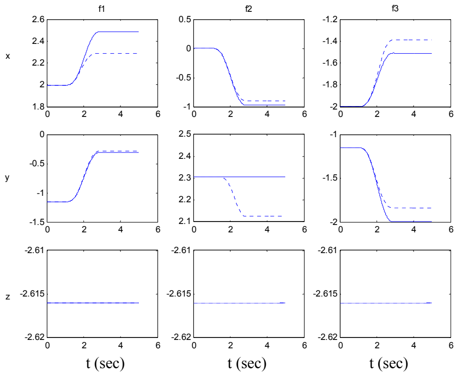
Figure 11. x-y-z components of the forces applied by the legs to the AGVs.
