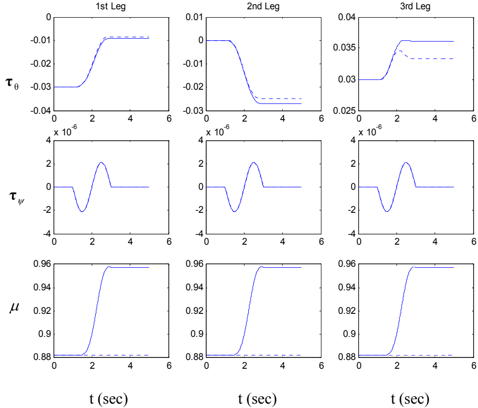
Figure 12. Required motor torques ( \tau_\theta and \tau_\psi ) and friction ( \mu ) for the three AGVs for the second maneuver.
