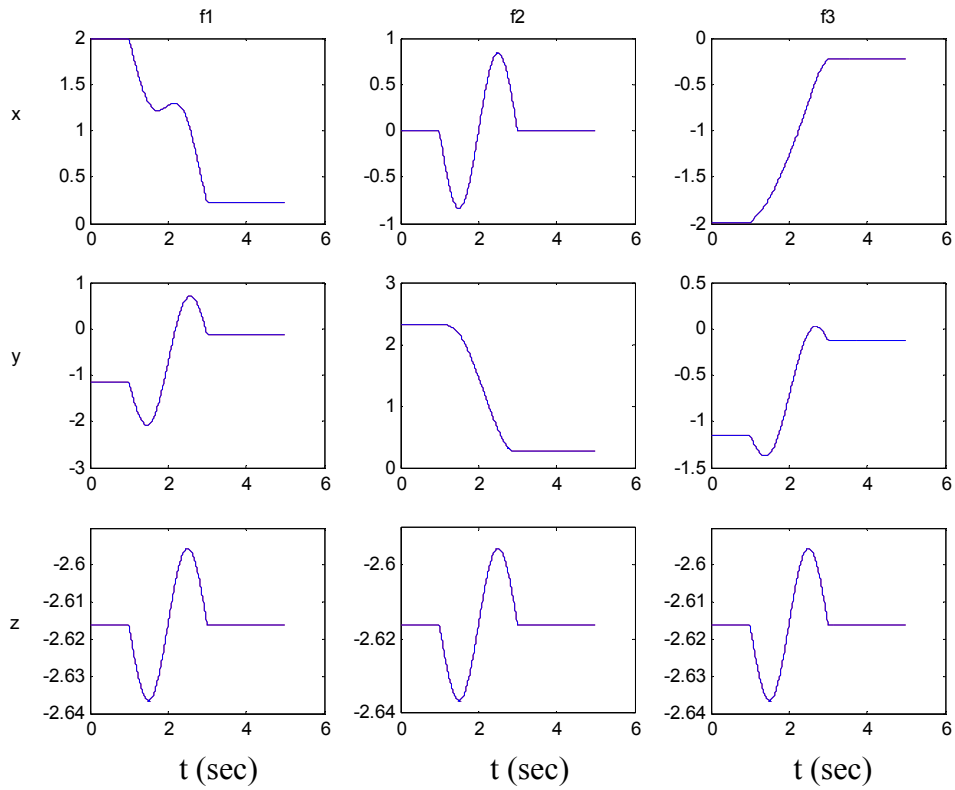
Figure 8. x-y-z components of the forces applied by each of the three legs to the AGVs
