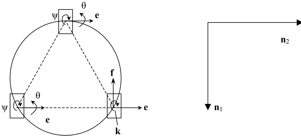
Figure 5. Top view of the Synchro-drive AGV. In this figure, \psi = -\pi/2 .
