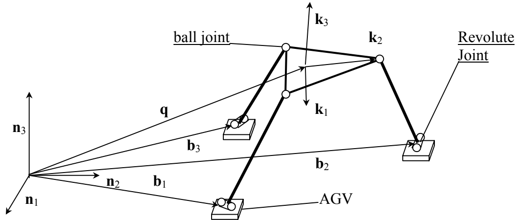
Figure 1. 3-D Representation of the System.
