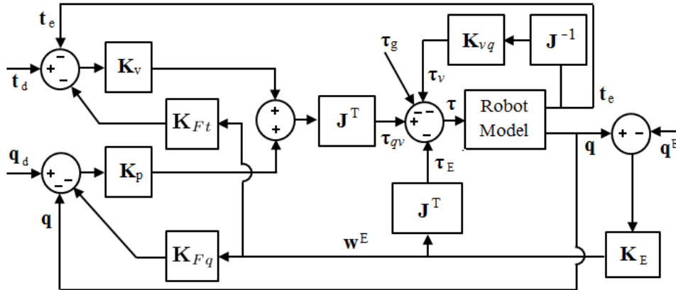
Figure 3 Impedance control model
