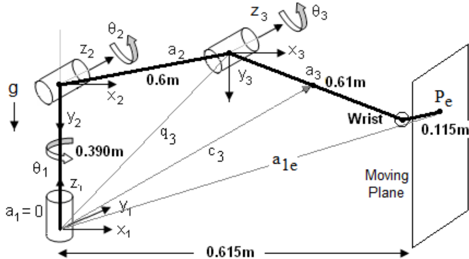
Figure 9 Architecture of KUKA KR5 arc robot
