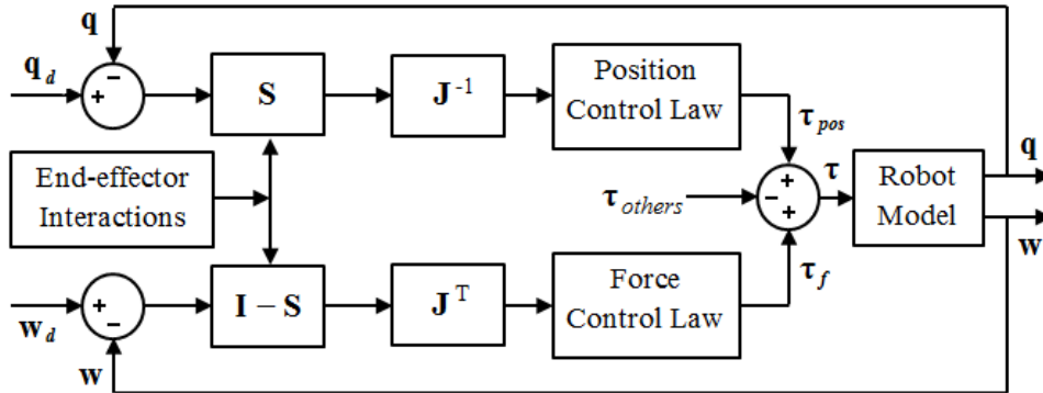
Figure 5 Hybrid control model
