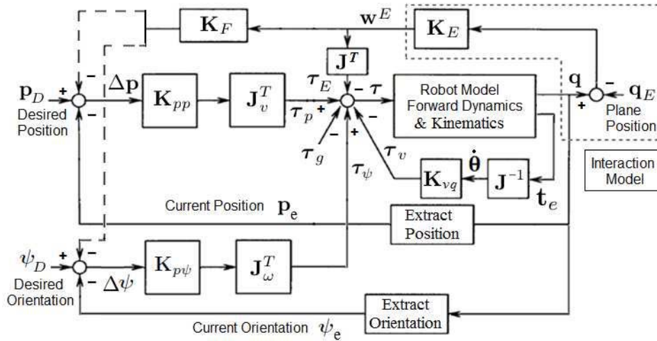
Figure 2 Stiffness control model
