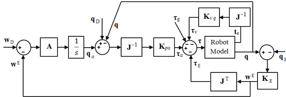
Figure 4 Admittance control model
