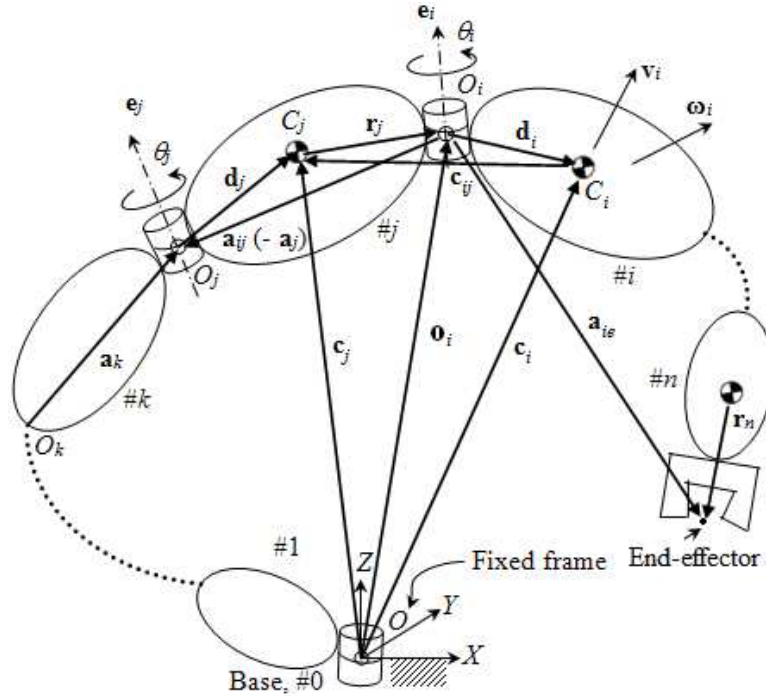
Figure 1 A serial chain system
